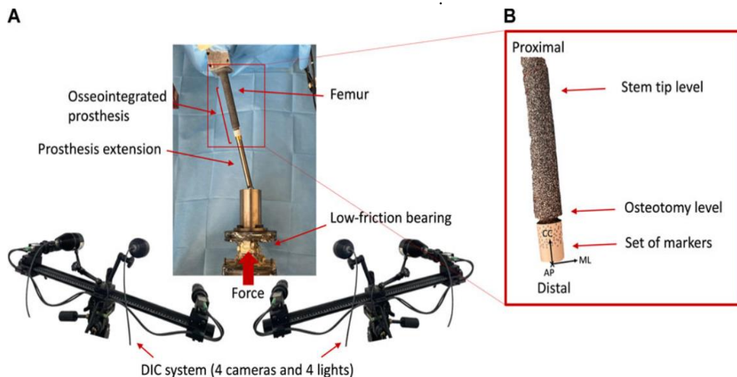
Fig. 4. Primary stability assessment system
