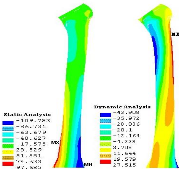
Fig. 5. Estimation of the peak load of the femur during tripping
