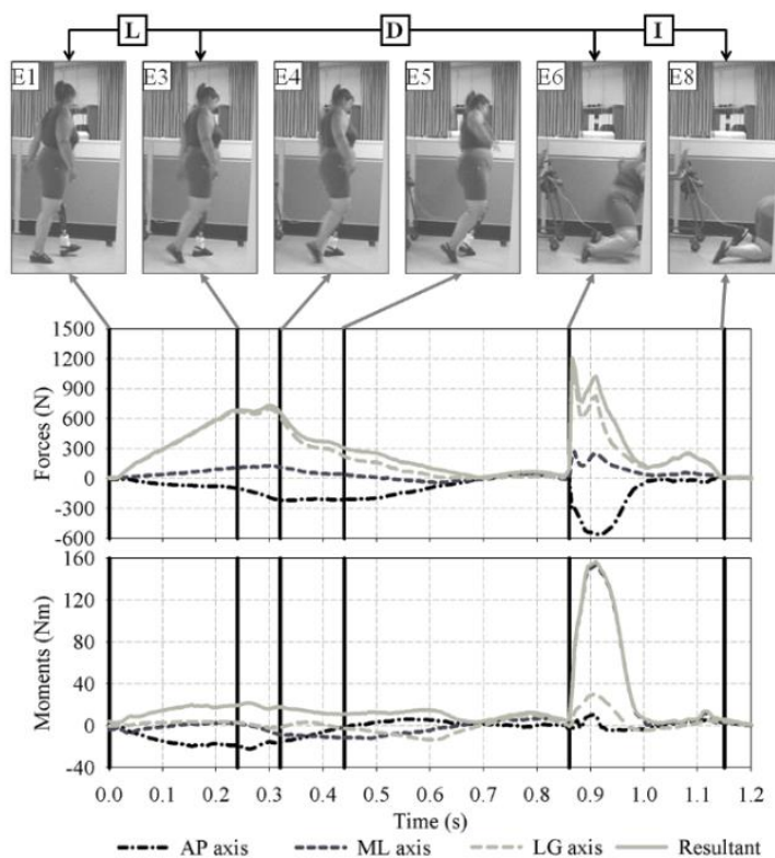
Fig. 6. Overview of the resultant force (R) and the three components of forces and moments along the antero-posterior (AP), medio-lateral (ML) and longitudinal (LG) axes of fixation during the loading (L), descent (D) and impact (I) phases of a forward fall, defined according to the sequence of events
