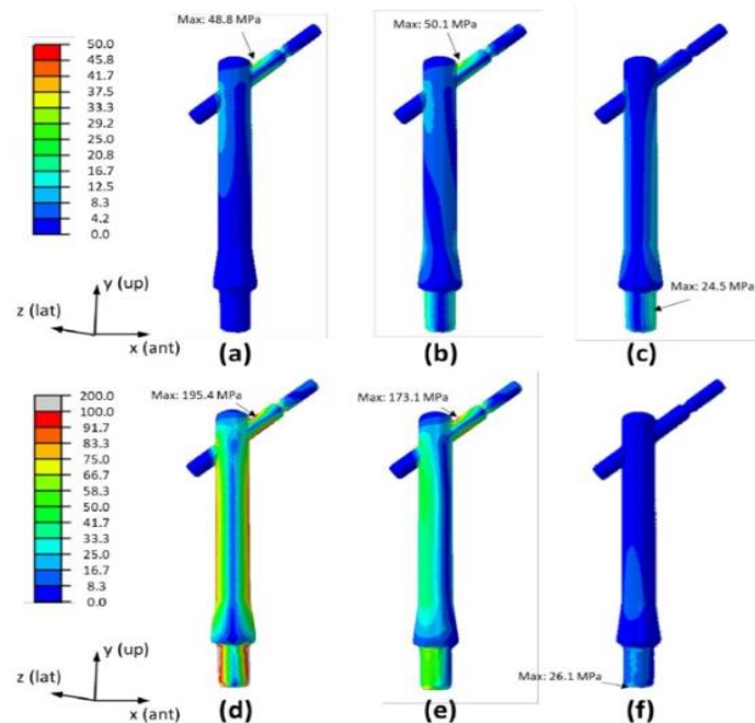
Fig. 3. The osseointegrated implant experienced the highest loads at the interface between the intramedullary post and screw and the abutment during walking
